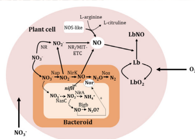
Nitric oxide (NO) and nitrous oxide ( \text{N}_2\text{O} ) metabolism in soybean nodules
