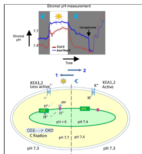
A working model for Arabidopsis KEA1 and KEA2 function in stroma pH regulation. Upon transition from dark to light, light-driven electron transport chain (ETC) acidifies the thylakoid lumen and causes alkalinization of the stroma. Upon transition from light to dark, the electron transport stops, and pH gradients are dissipated. Our results show that the stroma is predominantly neutralized by KEA1 and KEA2 via rapid influx of protons from the cytosol in exchange for \text{K}^+
